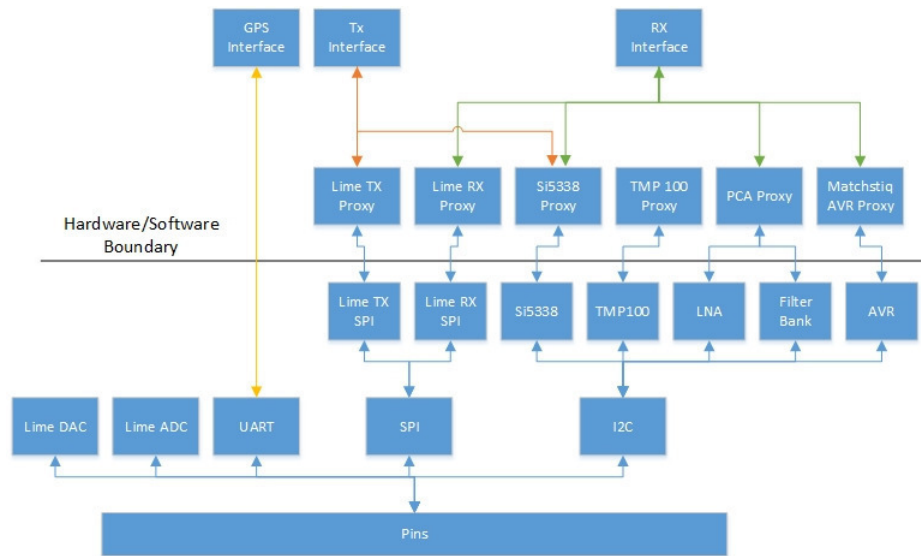
Figure 2: Device Worker & Proxy Diagram
