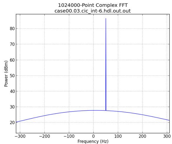
Figure 10: Frequency Domain: 50 Hz
