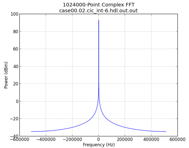
Figure 6: Frequency Domain: 0 Hz
