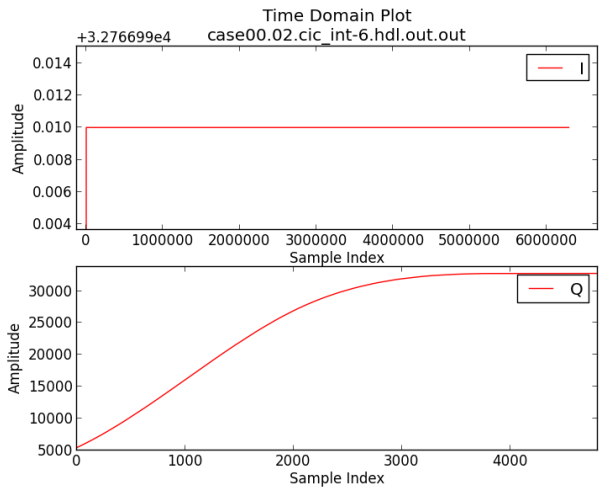
Figure 5: Time Domain: DC with amp=32767
